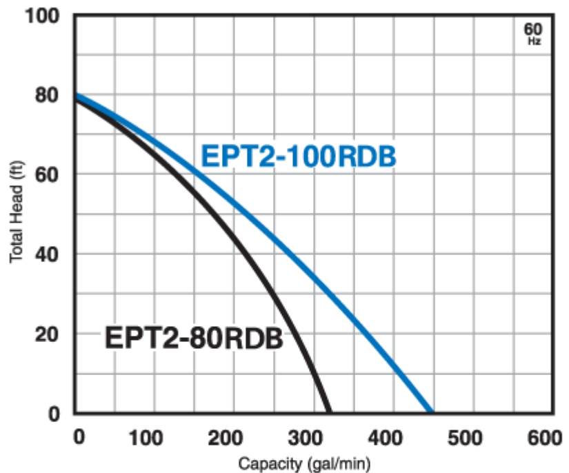
Performance Range
