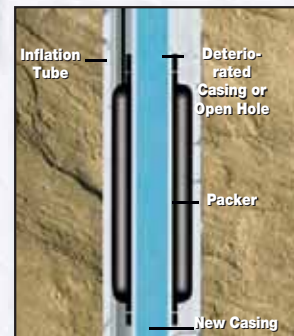
Relining Deteriorated Casing
